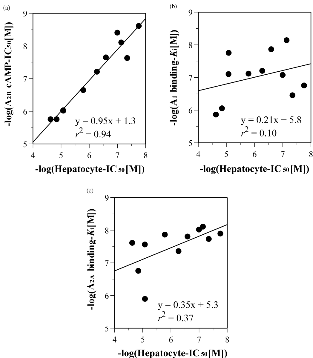
Figure 1. Correlation between inhibitory activities on NECA-induced glucose production in primary cultured rat hepatocytes and (a) inhibitory activities on NECA-induced cyclic AMP accumulation in CHO.K1 cells, (b) A 1 binding affinities, and (c) A 2A binding affinities (least-squares regression analysis).
