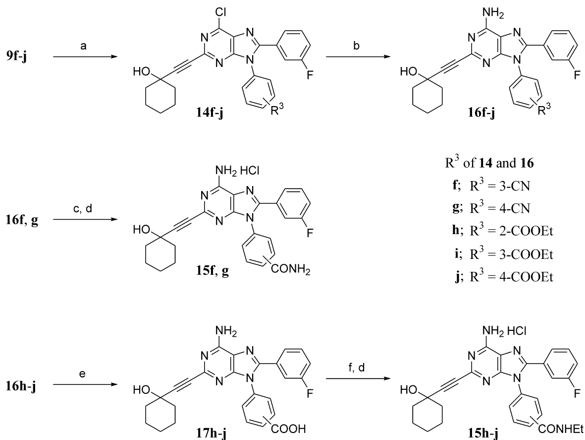
Scheme 3. Synthesis of 9-( N -ethyl)benzamidoadenine derivatives. Reagents: (a) 1-ethynyl-1-cyclohexanol, (PPh 3 ) 2 PdCl 2 , CuI, Et 3 N/THF; (b) NH 3 /EtOH; (c) NaOH, H 2 O 2 /CHCl 3 -MeOH-H 2 O; (d) HCl/MeOH or EtOH; (e) NaOH/CHCl 3 -MeOH-H 2 O; (f) EtNH 2 ·HCl, Et 3 N, WSC, HOBt/DMF.
