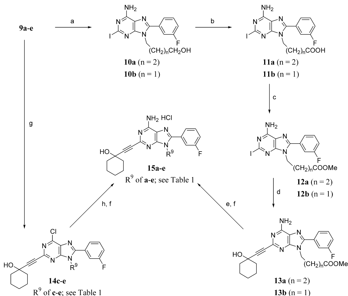
Scheme 2. Synthesis of 9-amidoalkyladenine derivatives. Reagents: (a) NH 3 /MeOH; (b) RuO 2 ·H 2 O, NaIO 4 /CH 3 CN–CHCl 3 –H 2 O; (c) SOCl 2 /MeOH; (d) 1-ethynyl-1-cyclohexanol, (PPh 3 ) 2 PdCl 2 , CuI, Et 3 N/DMF; (e) EtNH 2 /EtOH–H 2 O; (f) HCl/MeOH; (g) 1-ethynyl-1-cyclohexanol, (PPh 3 ) 2 PdCl 2 , CuI, Et 3 N/THF; (h) NH 3 /EtOH.
