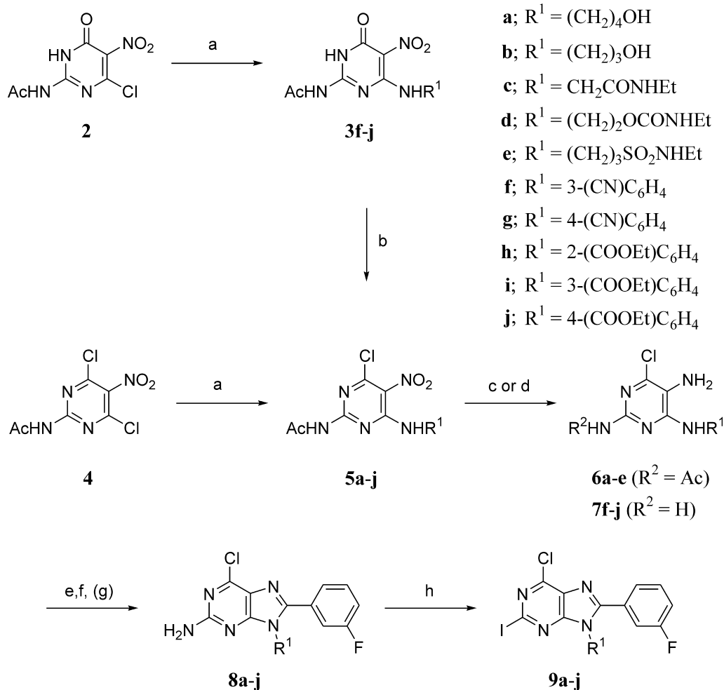
Scheme 1. Preparation of 8-aryl-6-chloro-2-iodopurine intermediates. Reagents: (a) R^1NH_2 , AcOH/THF (–MeOH); (b) POCl_3 , N,N -dimethylamine, Et_4NCl/CH_3CN ; (c) H_2 , Raney Ni/MeOH; (d) NaBH_4 , SnCl_2 \cdot 2H_2O/EtOH ; (e) 3-fluorobenzaldehyde, AcOH/MeOH; (f) FeCl_3/EtOH ; (g) HCl/H_2O –THF; (h) CH_2I_2 , isoamyl nitrite, CuI/THF.
